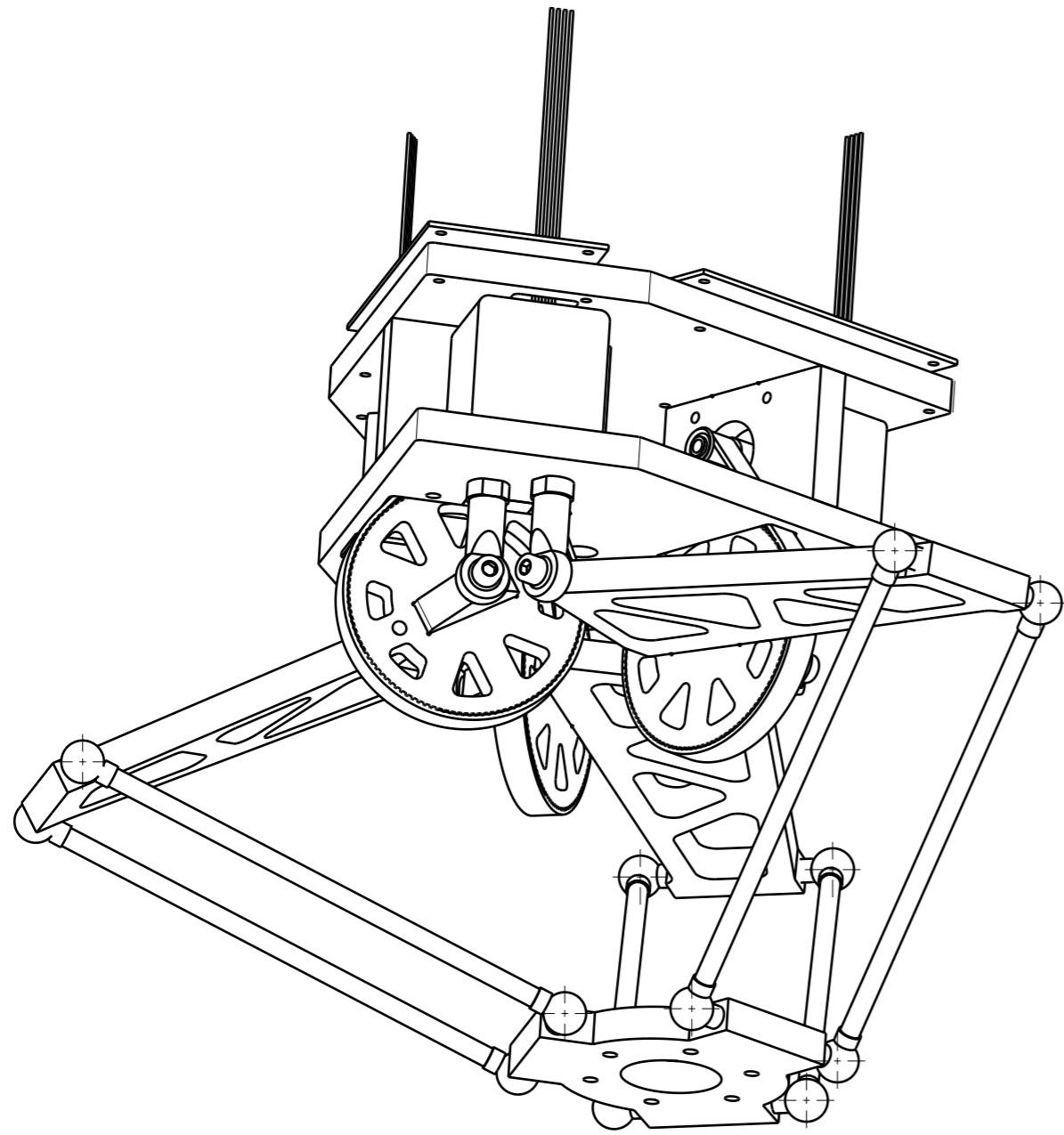
Isometric view Scale: 1:2
