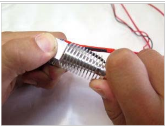
Heatsink is screwed down onto top of heatbreak.
