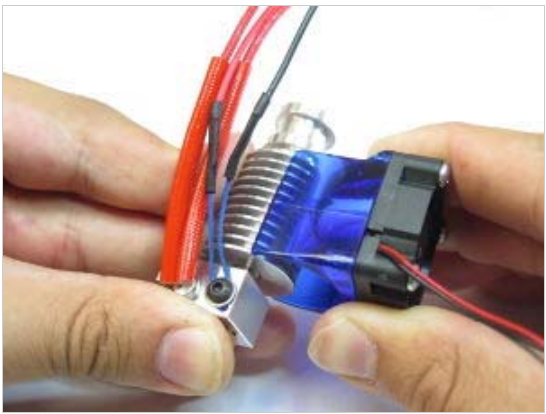
Fan duct clipping to heatsink.
