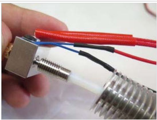
PTFE going down into Heat Break.
