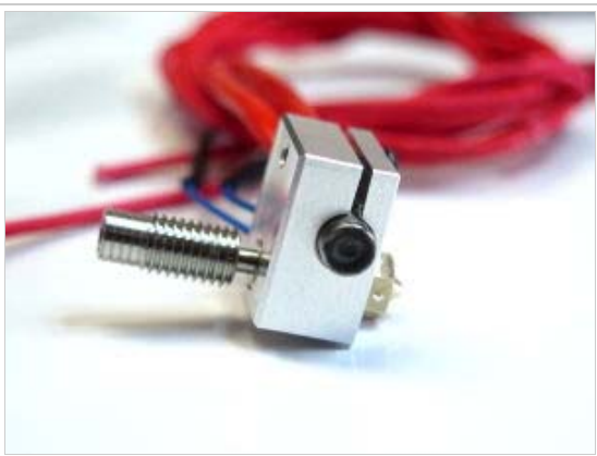
HeaterBlock tightened around cartridge.
